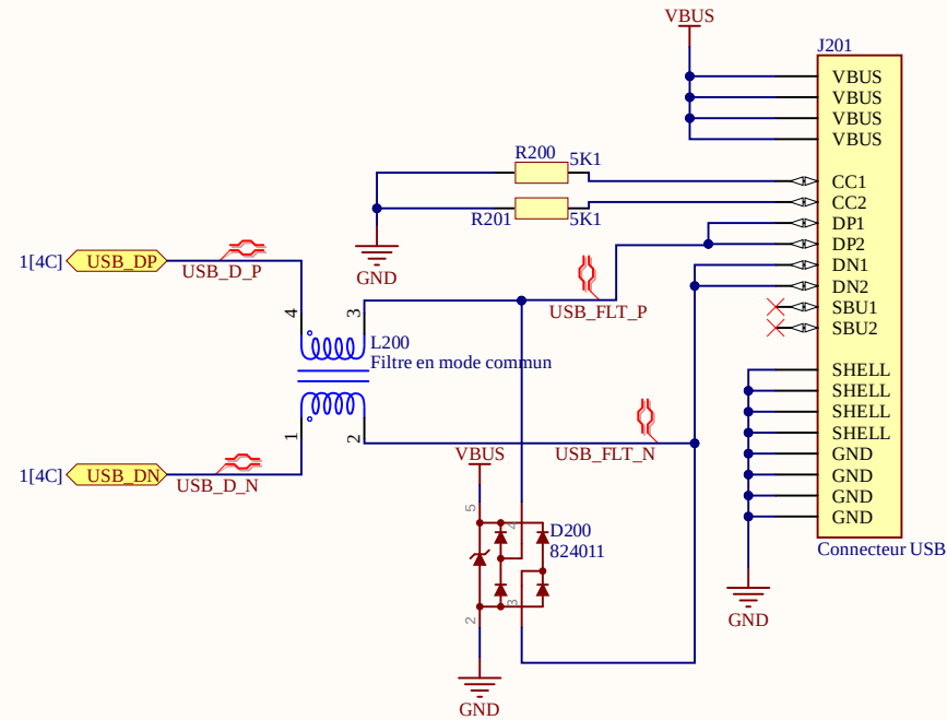
Connection USB
