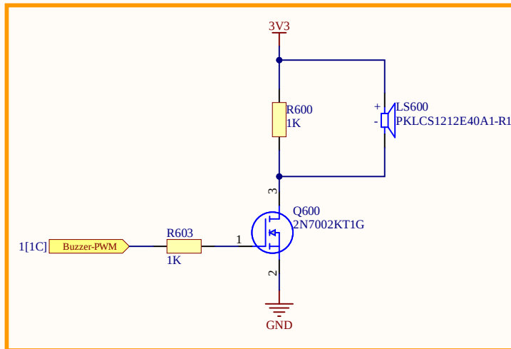
Pilotage buzzer
